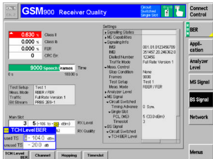
Fig. 23 BER Measurement
