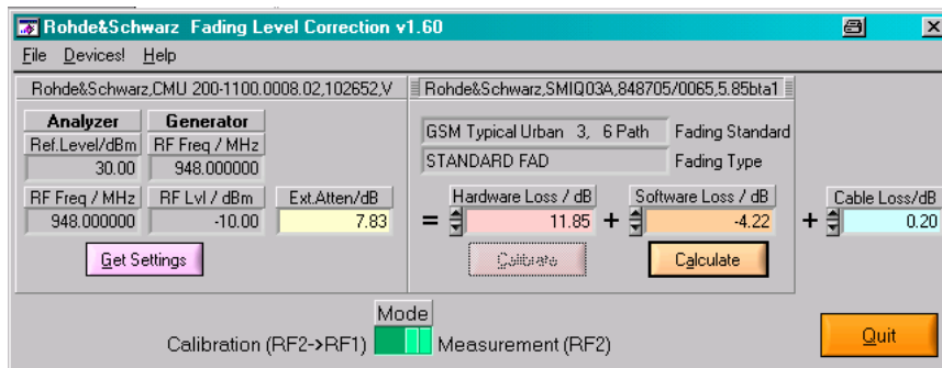
Fig. 19 Main Window Measurement Mode
