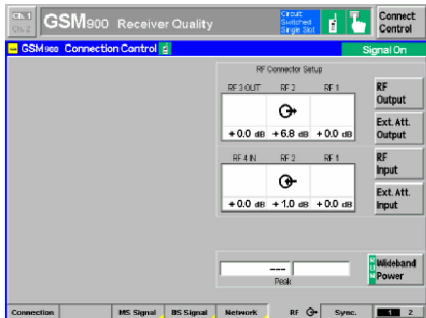
Fig. 22 Connection Control
