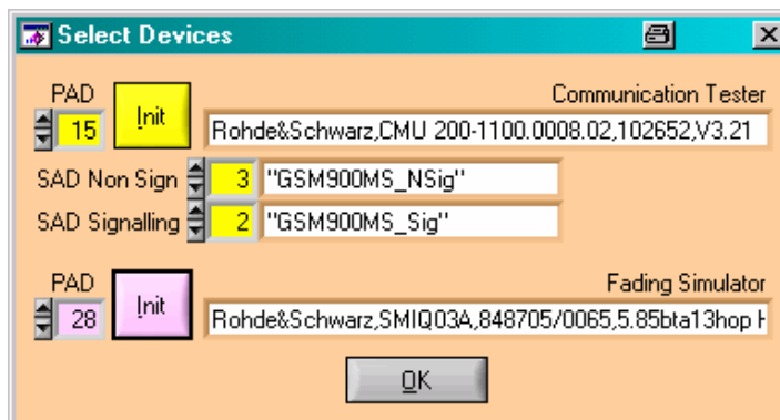
Fig. 14 Select Devices
