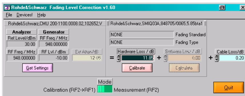
Fig. 15 Program Window
